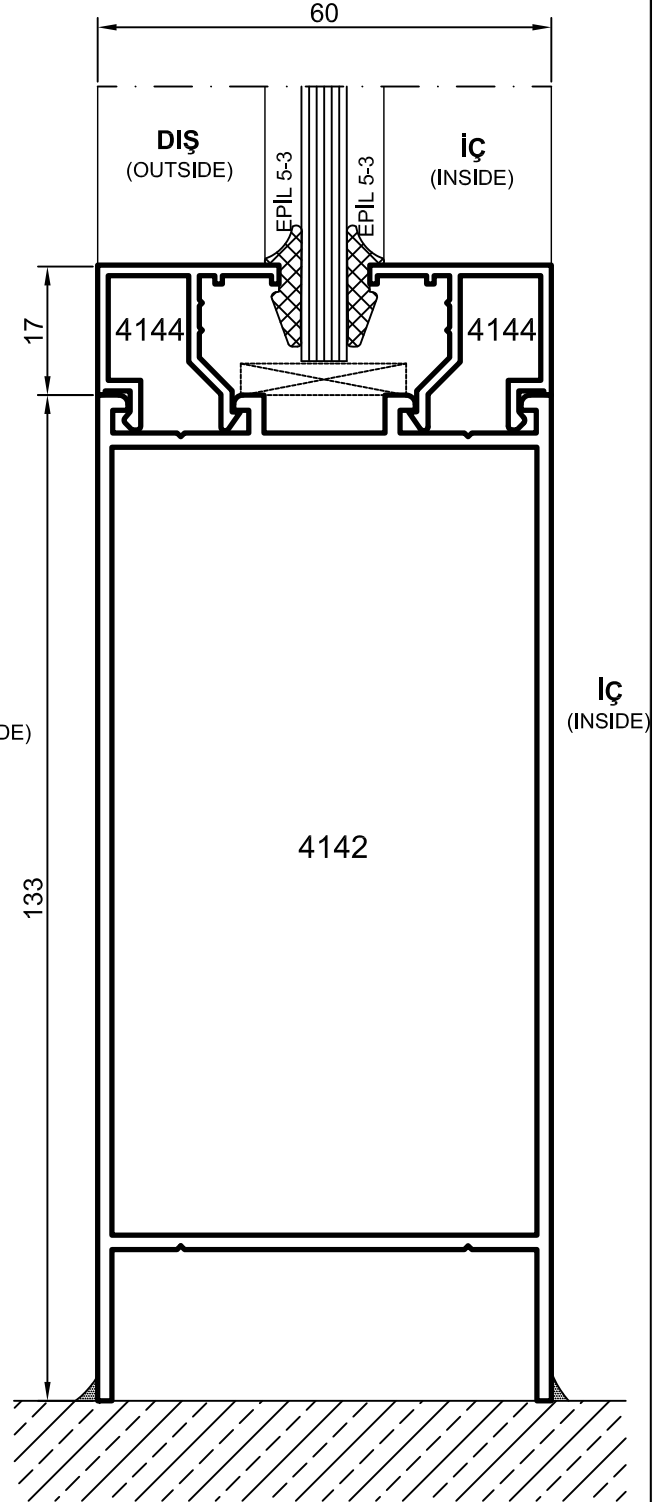
Detay Detail 5
