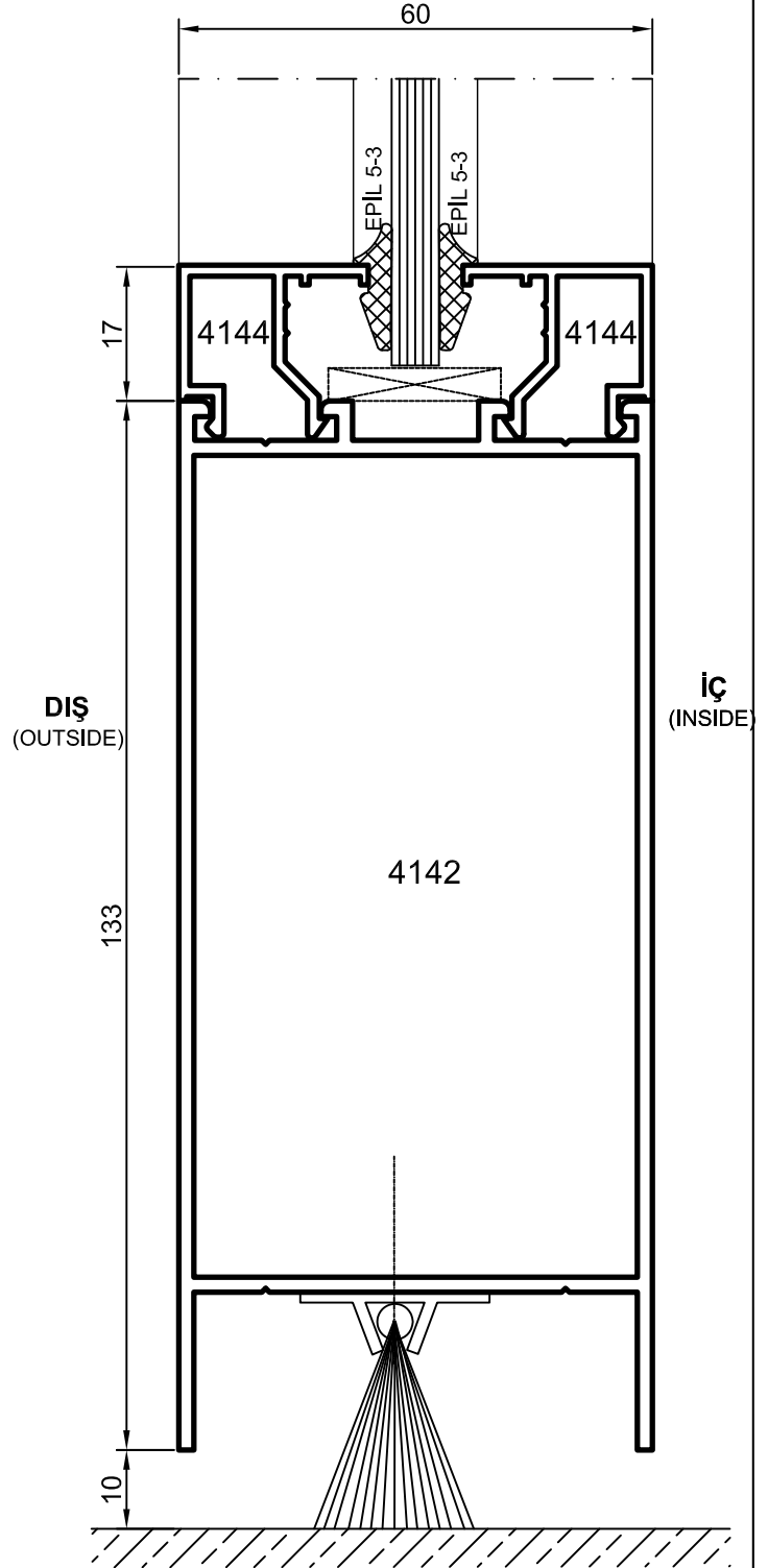
Detay Detail 5
