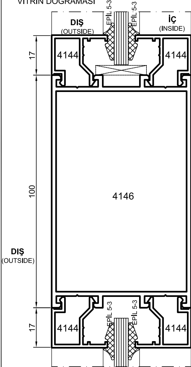
Detay Detail 4
